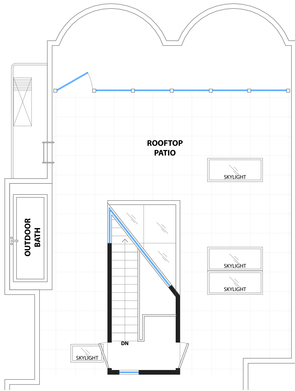
ROOFTOP LEVEL
